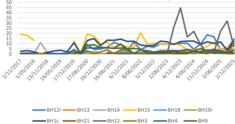
Chart 7: Dissolved Iron (mg/L)
