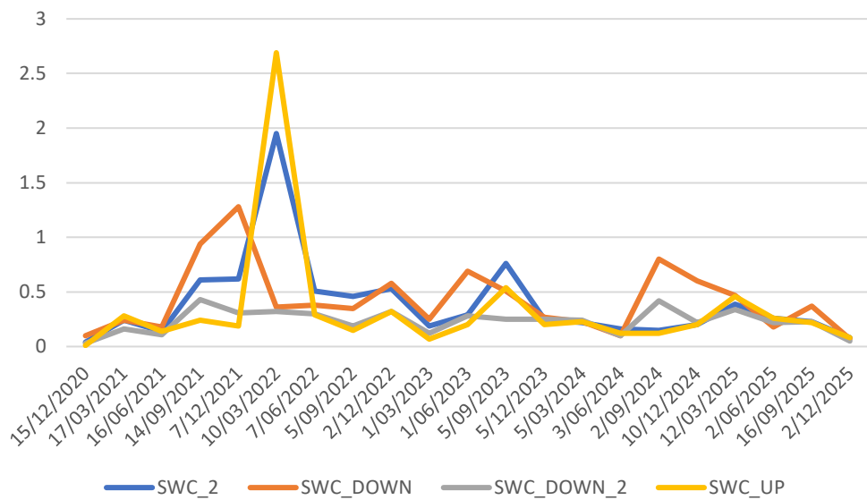
Chart 35: Ammonia as N (mg/L)
