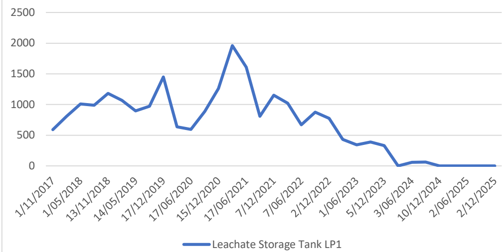
Chart 47: Ammonia as N (mg/L)
