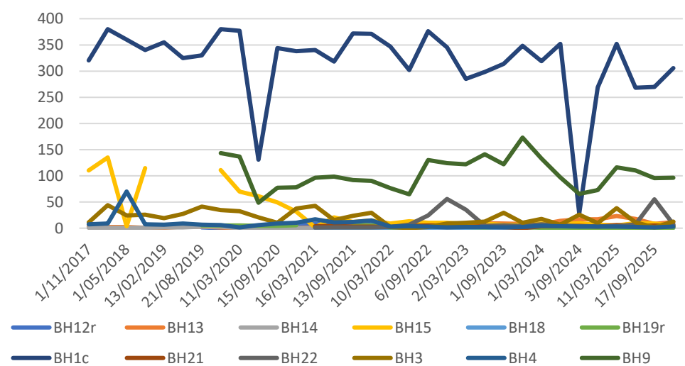
Chart 3: Ammonia as N (mg/L)
