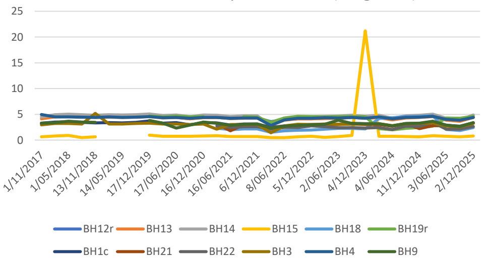
Chart 6: Depth to Water (mbgl TOC)
